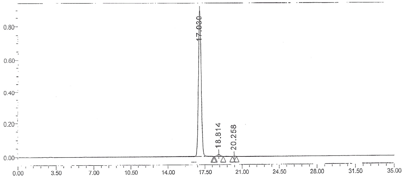
Auto-Scaled Chromatogram
